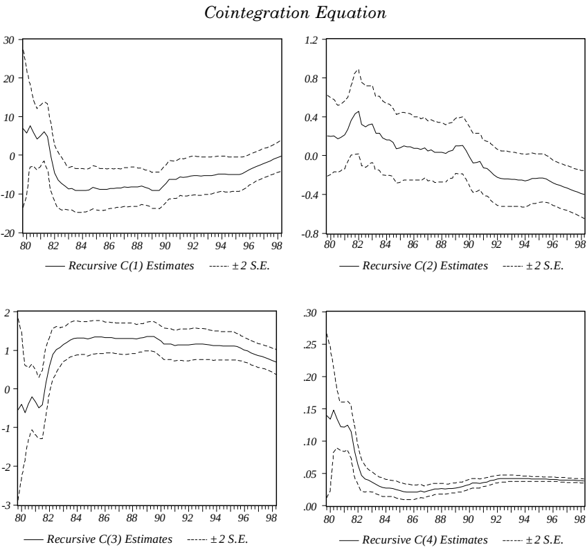
Figure B3. Recursive Estimation of Coefficients
