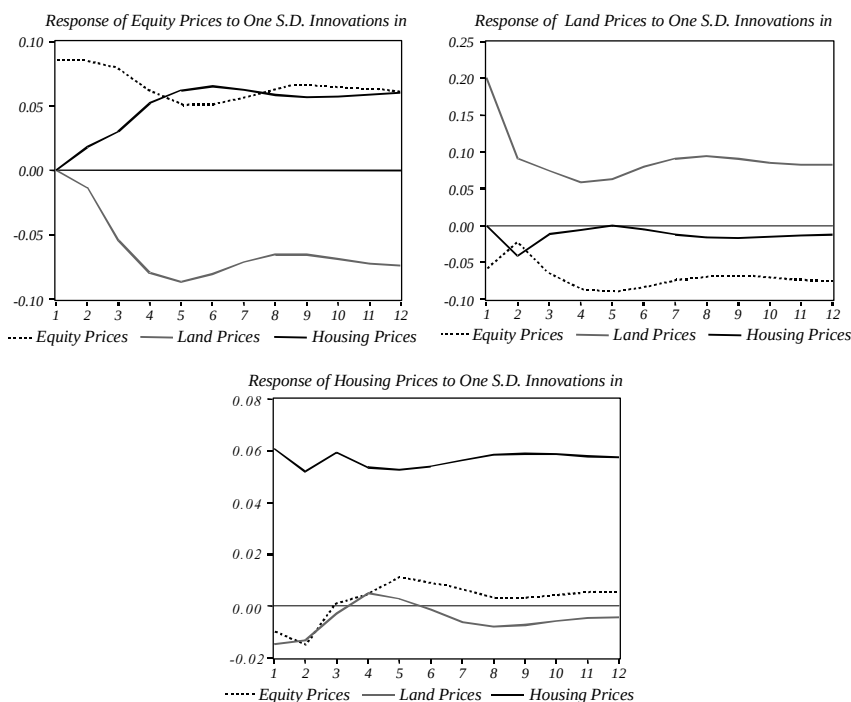
Figure 3. Impulse-Response Functions
