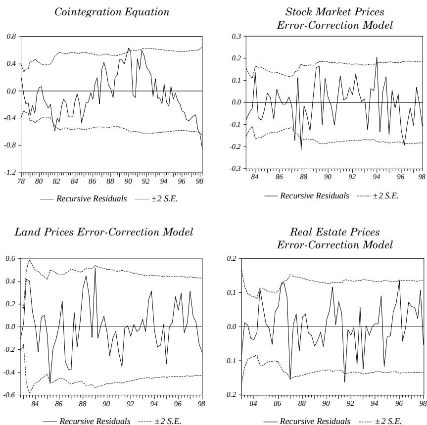
Figure B4. Recursive Residuals
