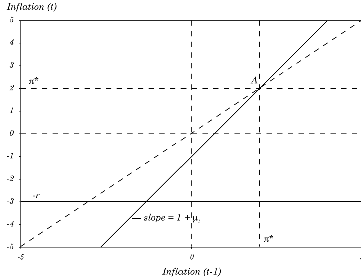
Figure 1. Inflation Dynamics, System Defined in Equations 1 and 2
