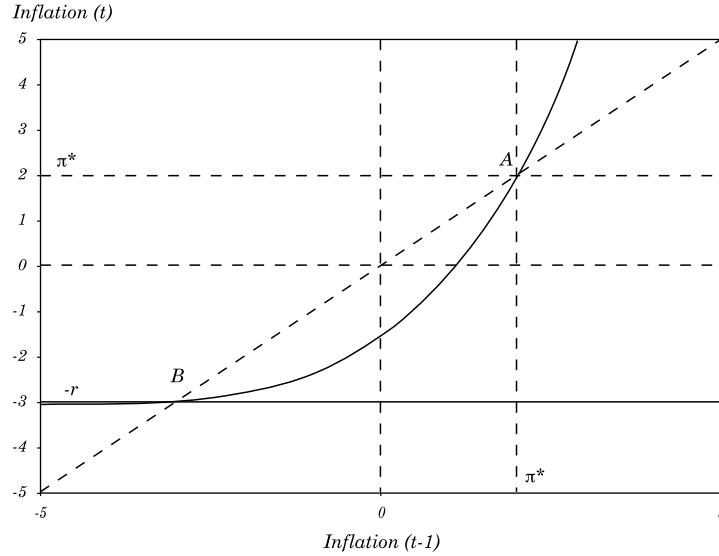
Figure 2. Inflation Dynamics, Nonlinear System
