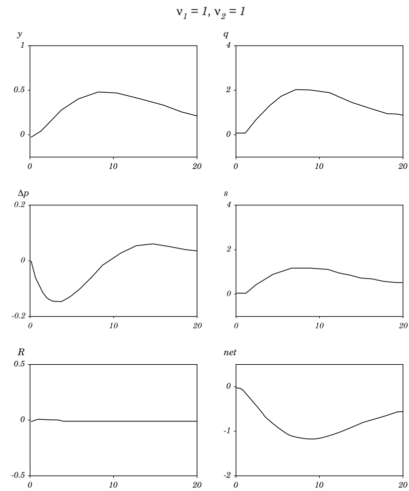
Figure 5. Responses to Unit Technology Shock to Policy Rule in Equation 39
